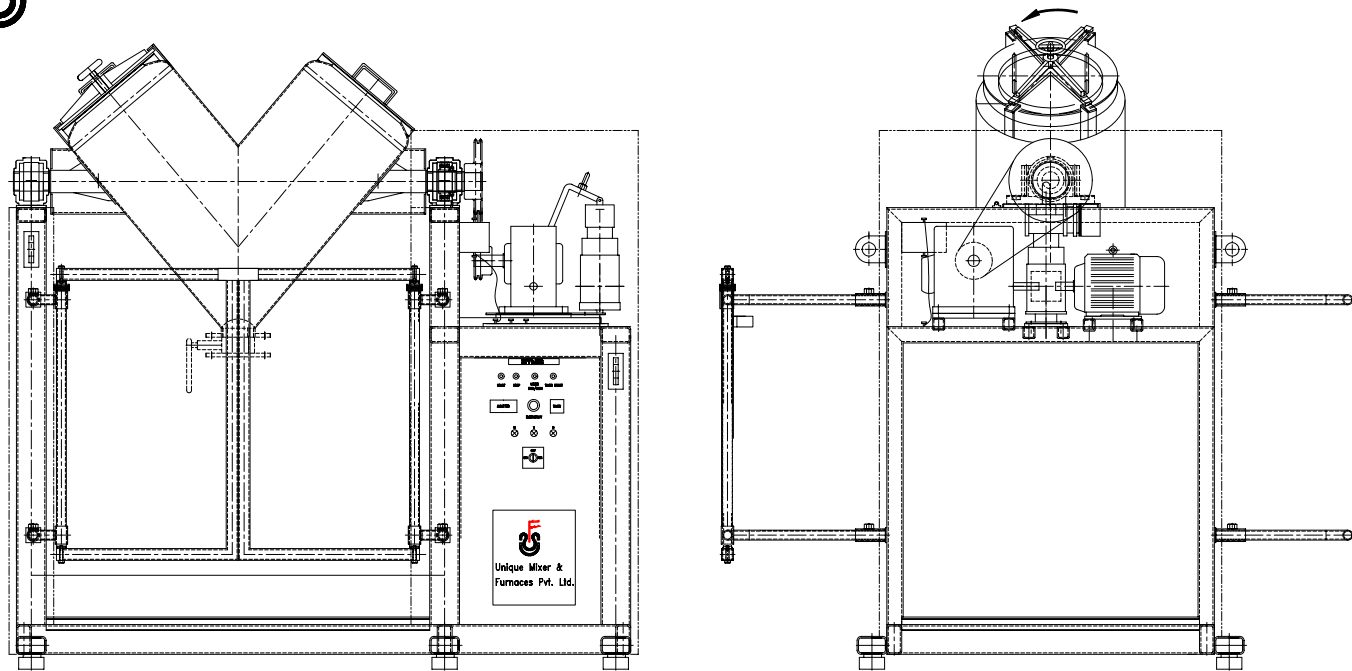
GENERAL ASSEMBLY OF V-BLENDER
