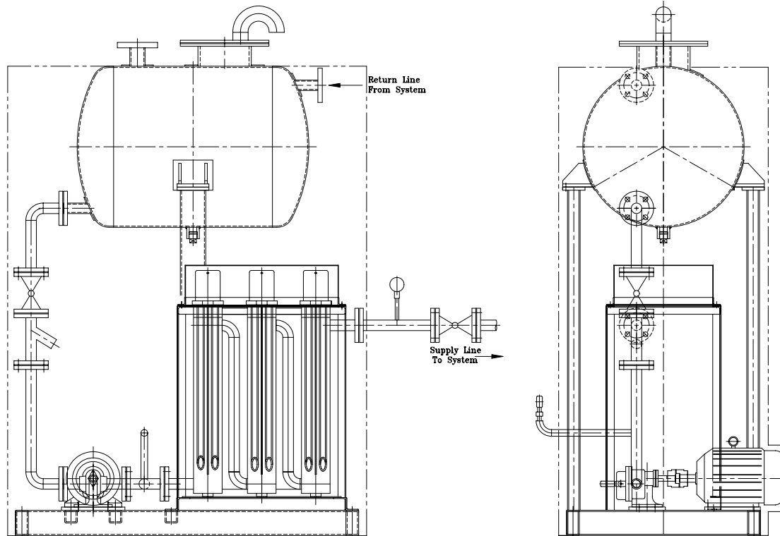
GENERAL ASSEMBLY OF THERMIC HEATING SYSTEM
