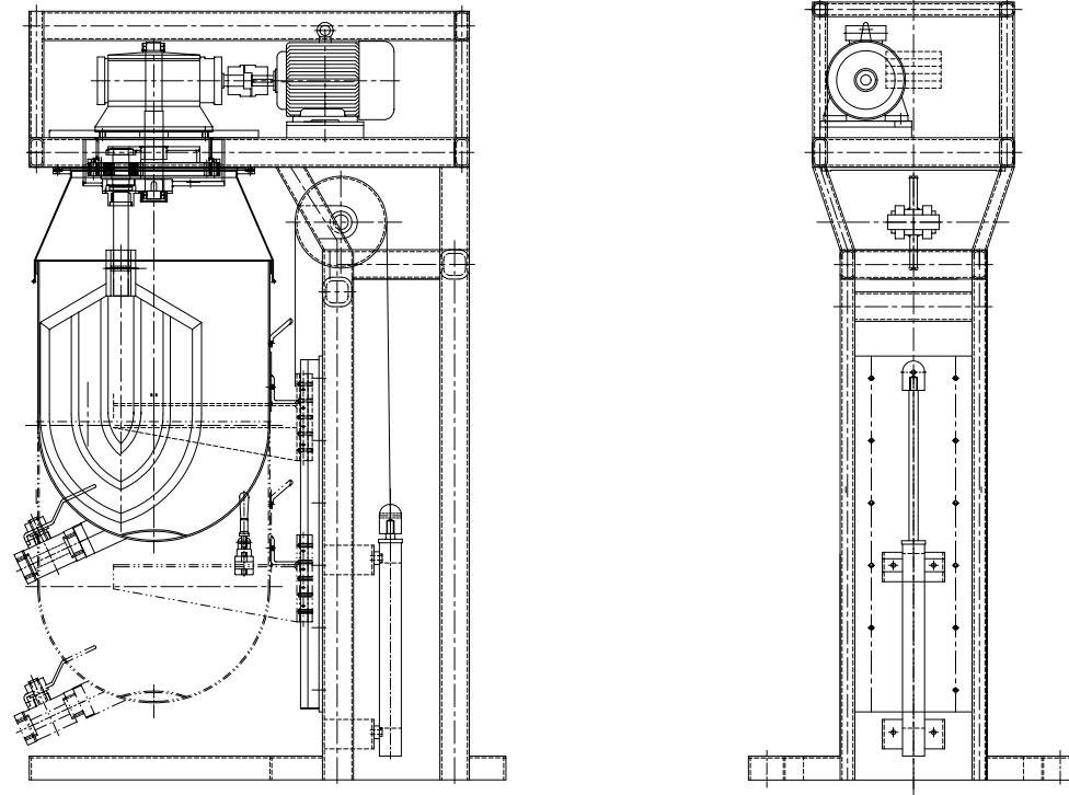
GENERAL ASSEMBLY OF SINGLE PLANETARY MIXER
