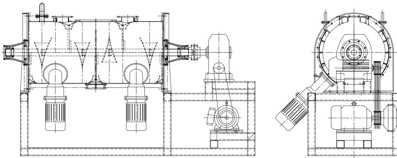
GENERAL ASSEMBLY OF PLOUGHSHARE MIXER
