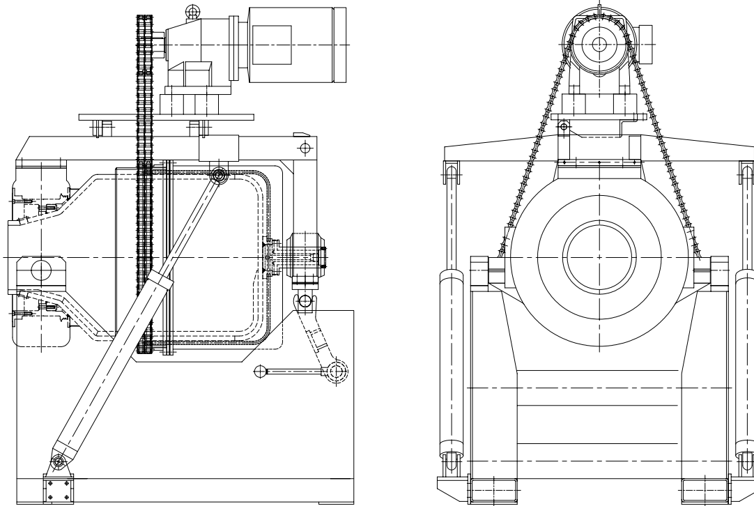
GENERAL ARRANGEMENT OF SPECIAL DUTY BALL MILL
